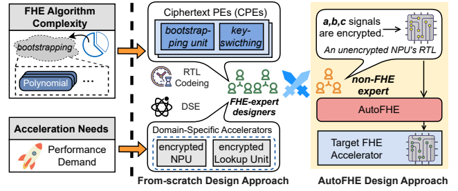
Fig. 1. The complexity of designing FHE processors, which relies on dual-domain expertise, and the proposed AutoFHE framework that automatically generates FHE processors.
